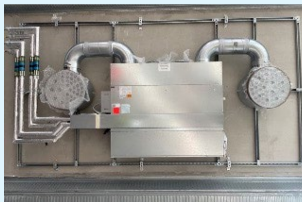
FIGURE 2 – Fan coil cassette secured to the soffit
